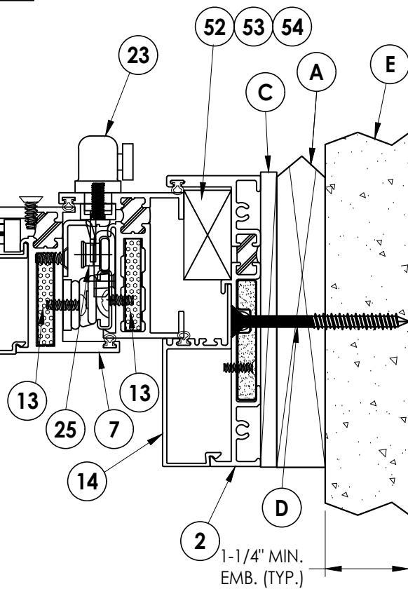
2 2 HORIZONTAL CROSS SECTION Shown w/ 1X Sub buck option
