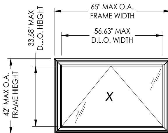
FRAME MOUNT
