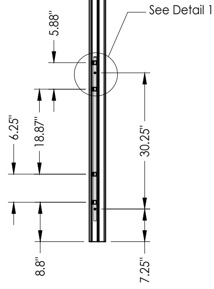
LOCK JAMB 2 Point Lock
