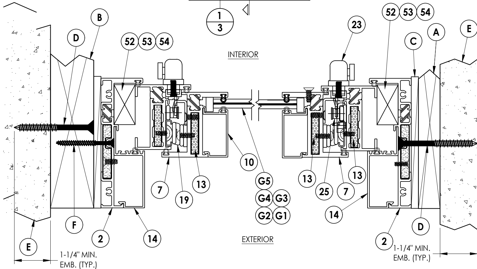
1 2 HORIZONTAL CROSS SECTION Shown w/ 2X Buck Construction
