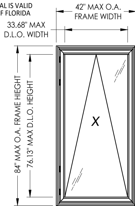
FRAME MOUNT
